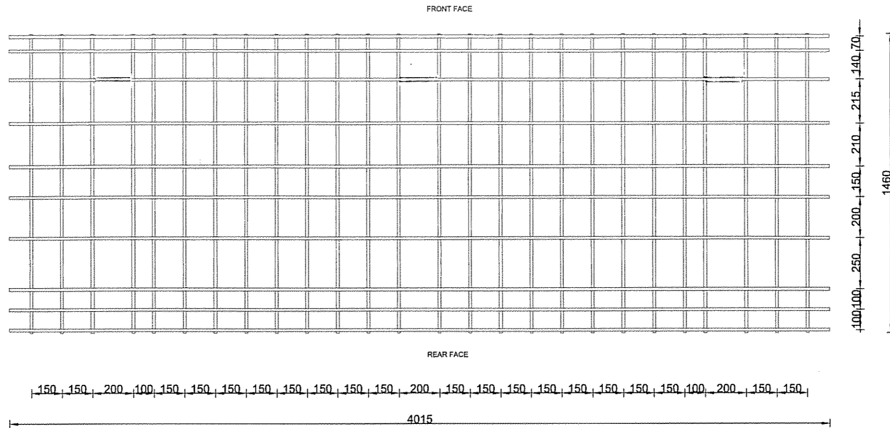
Customized dimensions of the grid of electro-welded mesh reinforcement placed in the Precast Segment ( Type A)
