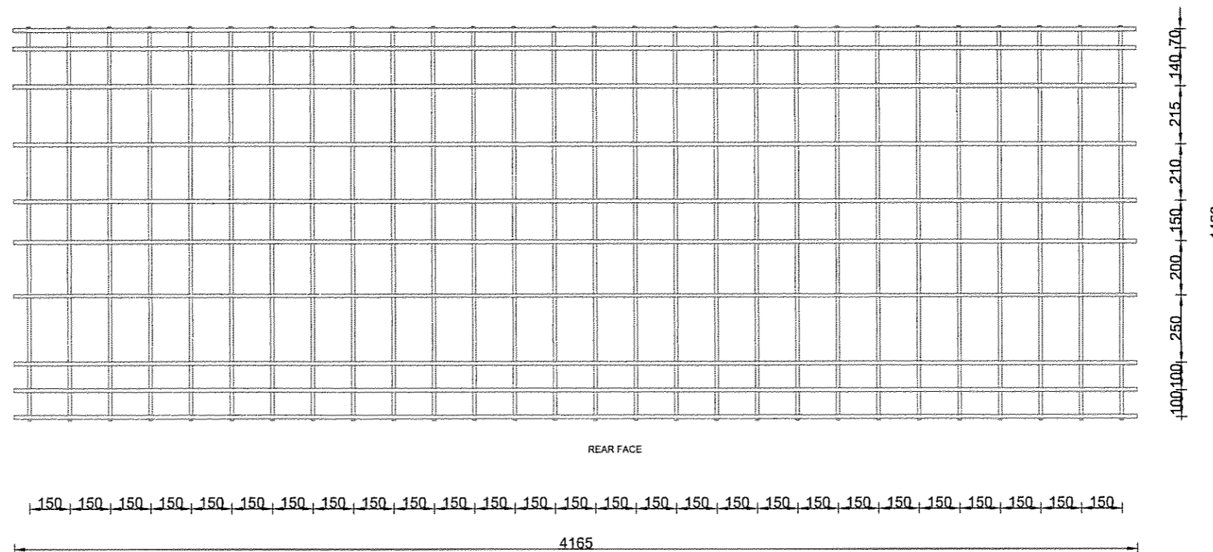
Customized dimensions of the grid of electro-welded mesh reinforcement placed in the Precast Segment ( Type A)
